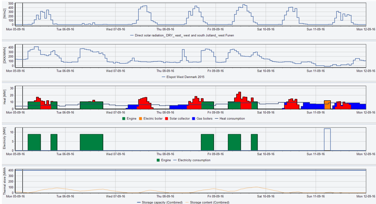
Figura 61: Modello EnergyPro (EMD international A/S)
